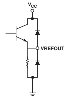
Figure 4. Reference Output
