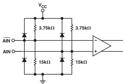
Figure 3. Analog Input
