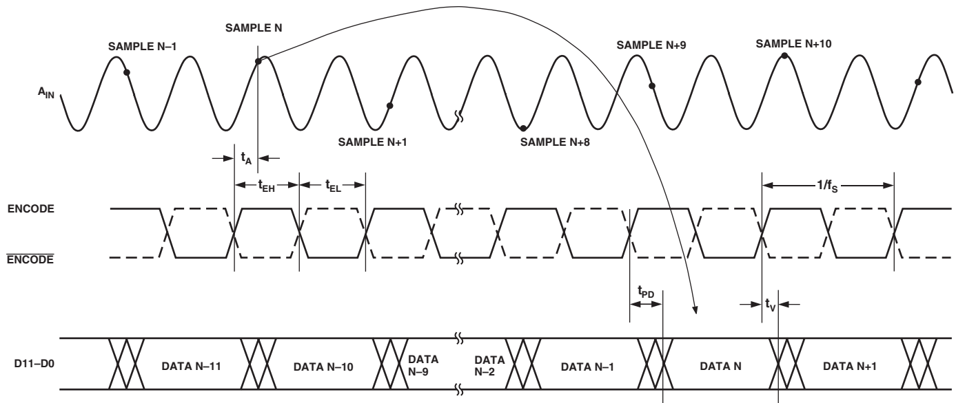
Figure 1. AD9433 Timing Diagram
